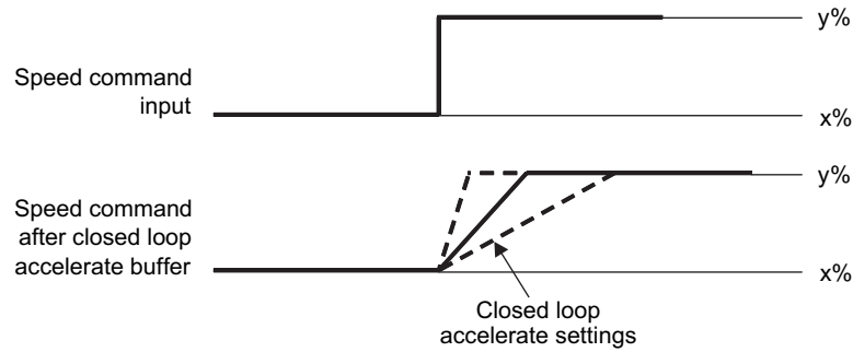
图 25. Closed-Loop Accelerate
