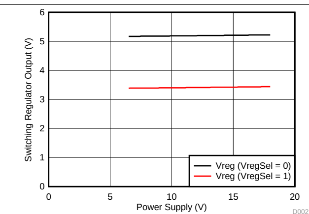
图 2. Step-down Regulator Output vs Power Supply
