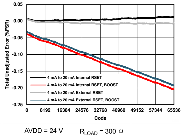
图 7-16. IOUT TUE vs Code (4 mA to 20 mA)
