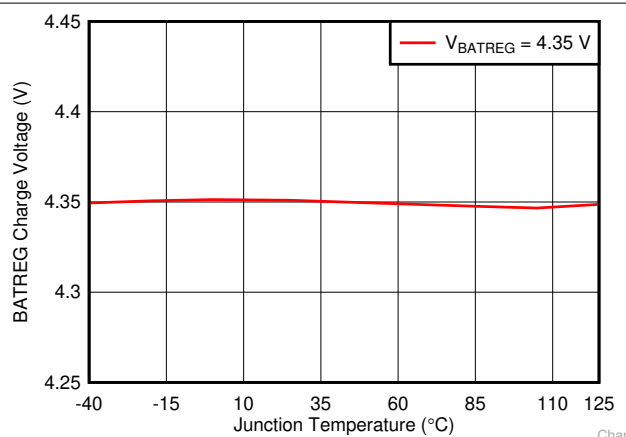
图 6-6. Battery Charge Voltage vs Junction Temperature
