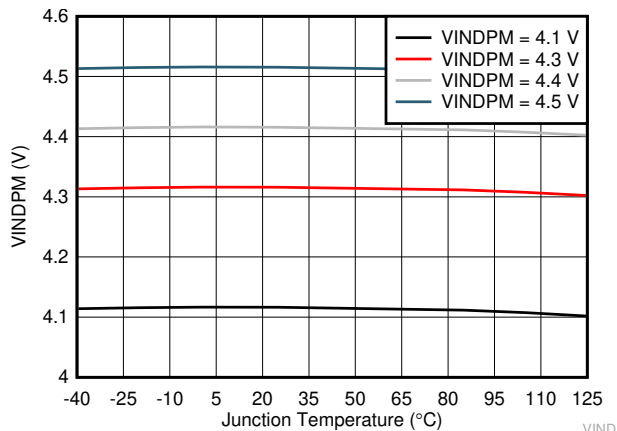
图 6-8. VINDPM vs Junction Temperature
