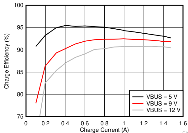
图 6-1. Charge Efficiency
