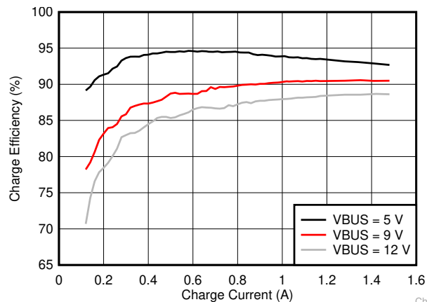
图 6-2. Charge Efficiency
