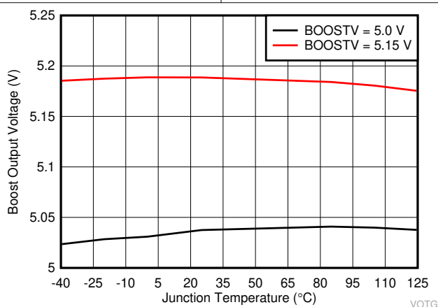
图 6-11. Boost Output Voltage vs Junction Temperature
