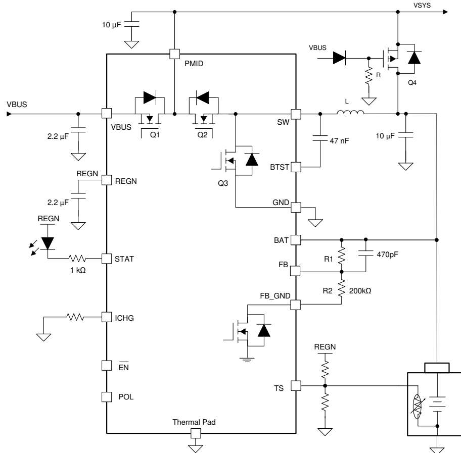
图 10-8. Typical Application Diagram with Power Path (1- \mu\text{H} inductor is recommended if maximum input voltage V_{\text{VBUS\_MAX}} < 6.2\text{V} ; 2.2- \mu\text{H} inductor is recommended if maximum input voltage V_{\text{VBUS\_MAX}} > 6.2\text{V} )
