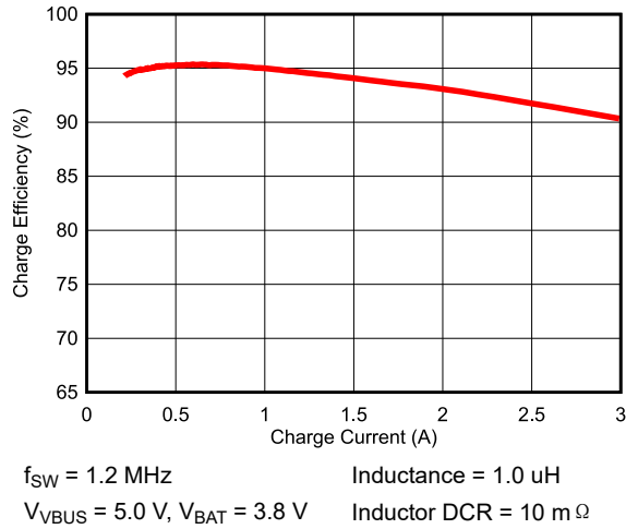
图 8-1. 1-Cell Battery Charge Efficiency vs. Charge Current
