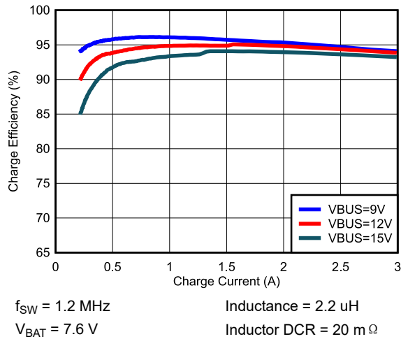
图 8-3. 2-Cell Battery Charge Efficiency vs. Charge Current
