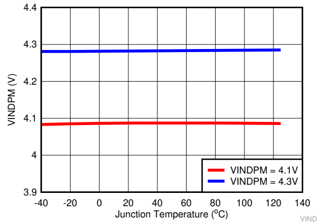
图 8-4. VINDPM vs. Junction Temperature
