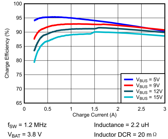
图 8-2. 1-Cell Battery Charge Efficiency vs. Charge Current
