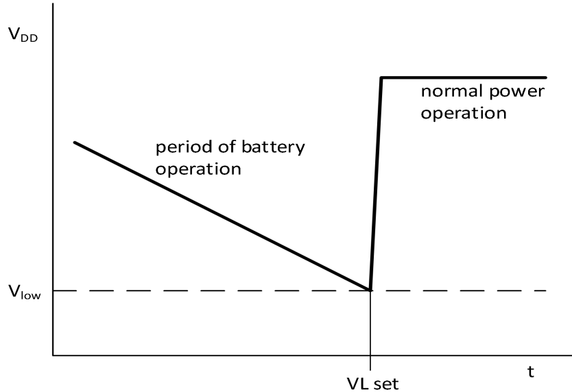
Fig 3. Voltage-low detection
