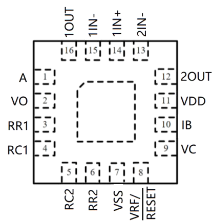
QFN-16 3*3
