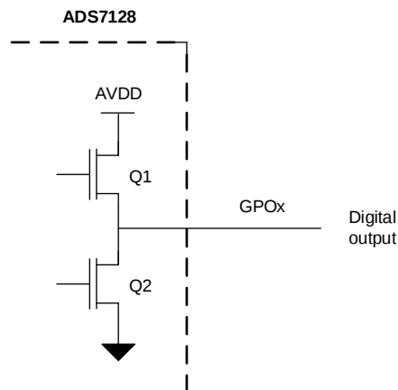
图 139. Digital Push-Pull Output
