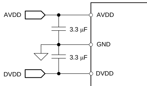
Figure 40. Power-Supply Decoupling
