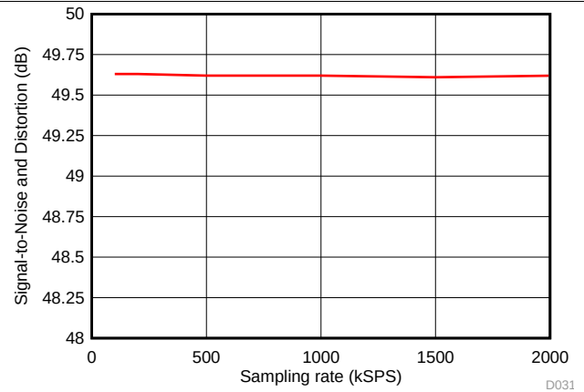
Figure 27. SINAD vs Sampling Rate
