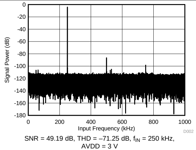
Figure 3. Typical FFT
