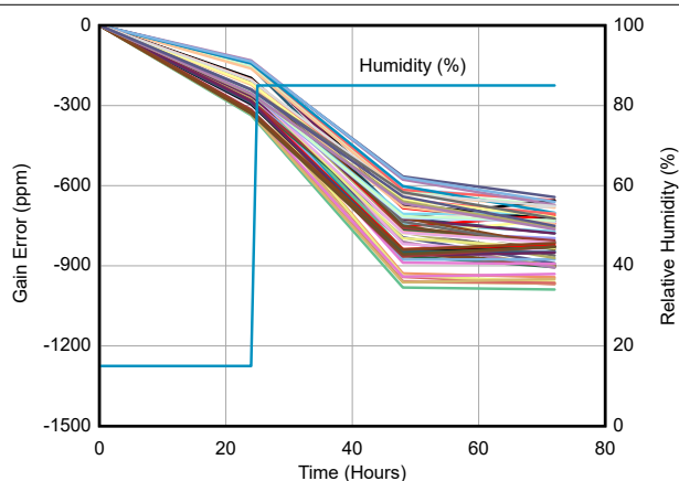
图 6-10. Gain Error vs Time (TSSOP Package)
