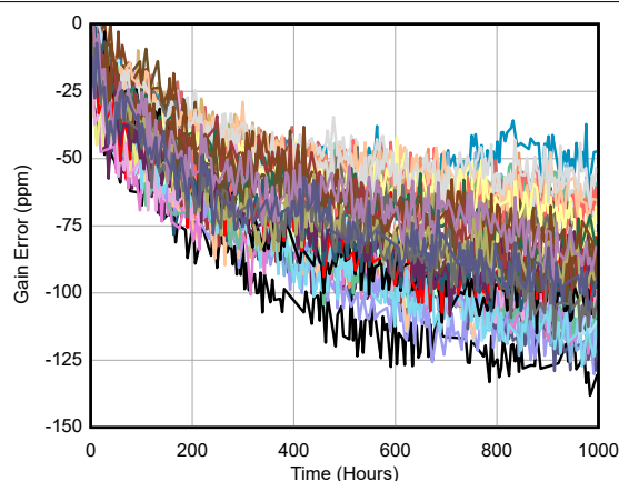
图 6-11. Gain Error vs Time (WQFN Package)
