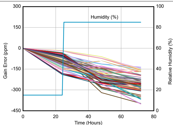
图 6-11. Gain Error vs Time (WQFN Package)
