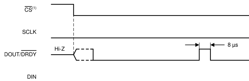
Figure 11. DOUT/DRDY Behavior Without Data Retrieval in Continuous-Conversion Mode
