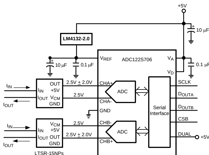
Figure 49. Interfacing the ADC122S706 to a Current Transducer
