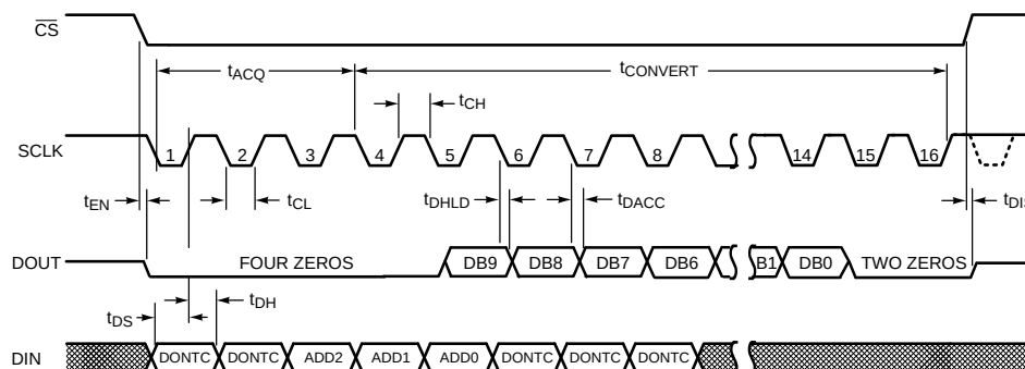
Figure 3. ADC088S102 Serial Timing Diagram
